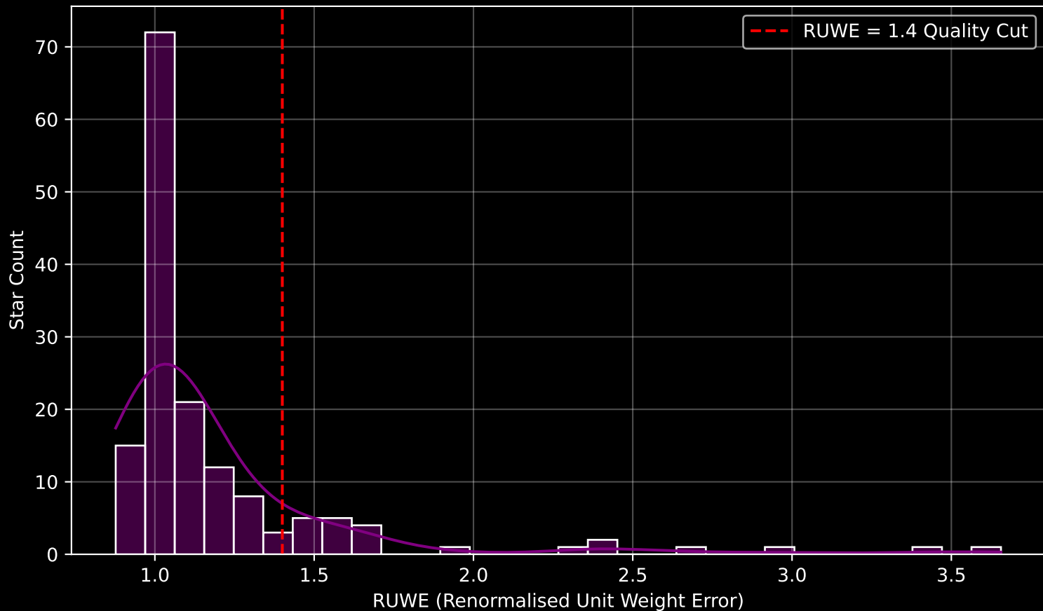
GAPOGEE DR17 Field [K2_C6_317+51_btx] RUWE Distribution (n= 153)
