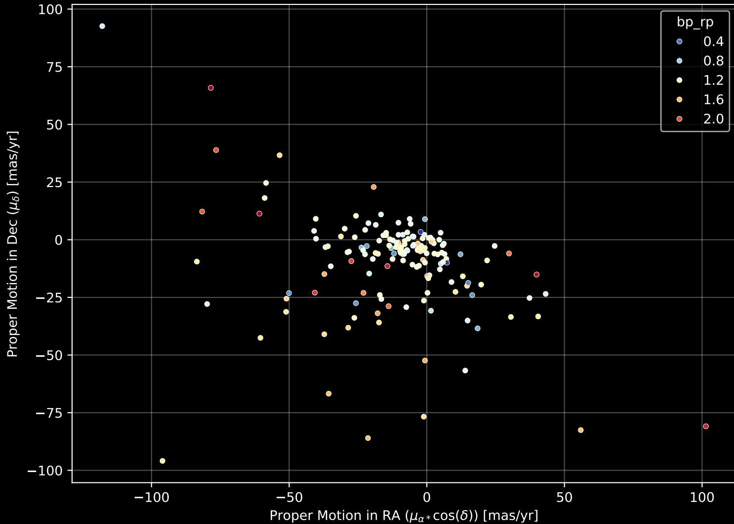
APOGEE DR17 Field: [K2_C6_317+51_btx] Proper Motion Diagram (n= 160)
